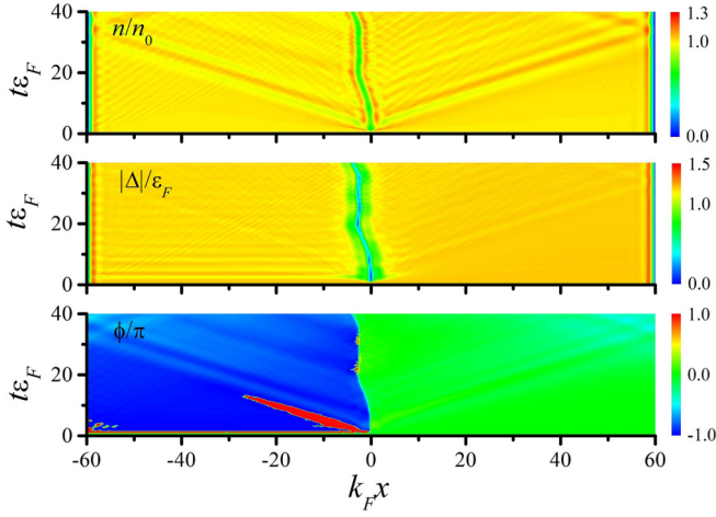
FIG. 11. Same physical quantities as in Fig. 2 in the Raman-type SOC Fermi superfluid. This dynamical simulation with only a single-component phase-imprinting strategy F_1 fails to produce a stable soliton in the BCS state ( h = 0.3\epsilon_F ).
