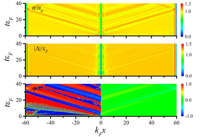
FIG. 7. Same physical quantities as in Fig. 2 in the Raman-type SOC Fermion superfluid in the BCS state ( h = 0.3\varepsilon_F ). With the phase-imprinting operation described by Eq. (24), the system is transformed from a ground state into a soliton state at time t\varepsilon_F = 1 .
