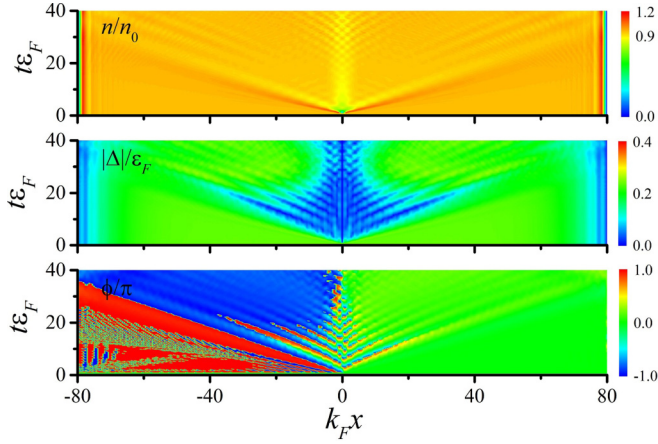
FIG. 9. Same physical quantities as in Fig. 2 in the Raman-type SOC Fermi superfluid in the topological state ( h = 1.1\varepsilon_F ). With the phase-imprinting operation described by Eq. (24), the system is transformed from a ground state into a Majorana soliton state at time t\varepsilon_F = 1 .
