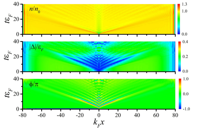
FIG. 10. Same physical quantities as in Fig. 2 in the Raman-type SOC Fermi superfluid in the topological state ( h = 1.1\varepsilon_F ). With the phase-imprinting operation described by Eq. (24), the system is transformed from a Majorana soliton state into a ground state at time t\varepsilon_F = 1 .
